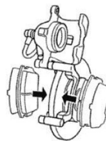
10 Introduce the new pads complete with respective plates.
