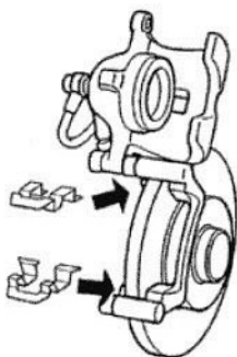
9 Replace the support plates.
