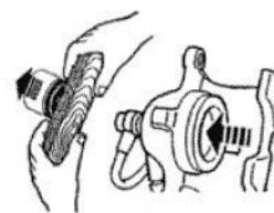
8 Push the piston back.
