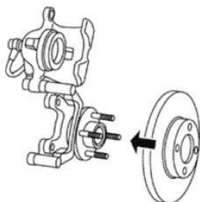
7 Fit the disc on the wheel hub.
