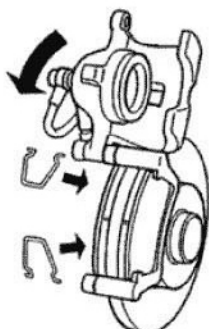
11 Insert the springs and turn the caliper.
